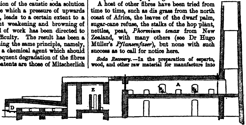
FIG. 14.—Porion Evaporator.
