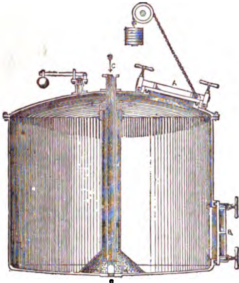
FIG. 1.—Section of Rag-Boiler.
