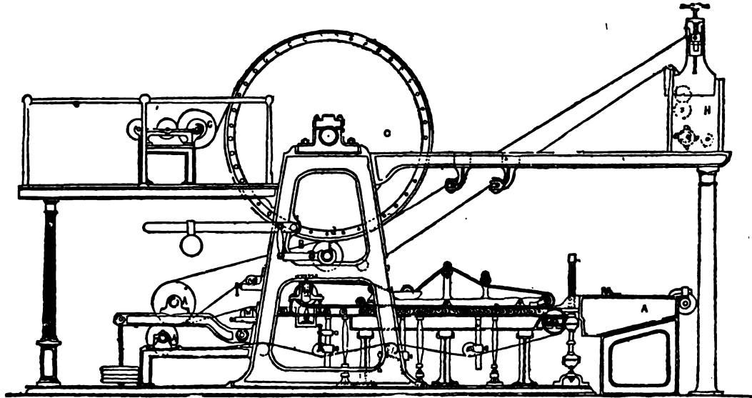
FIG. 6.—Single-Cylinder Machine.
