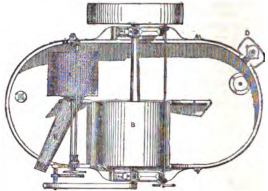
FIG. 3.—Breaking Engine—Horizontal Section.
