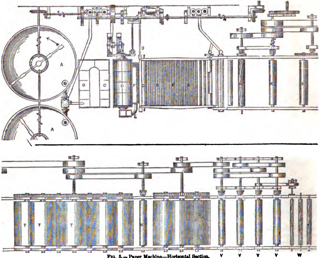
FIG. 5.—Paper Machine—Horizontal Section.
