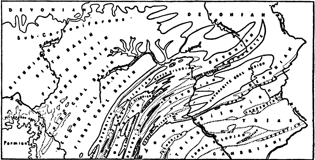
Geological Map of Pennsylvania.
