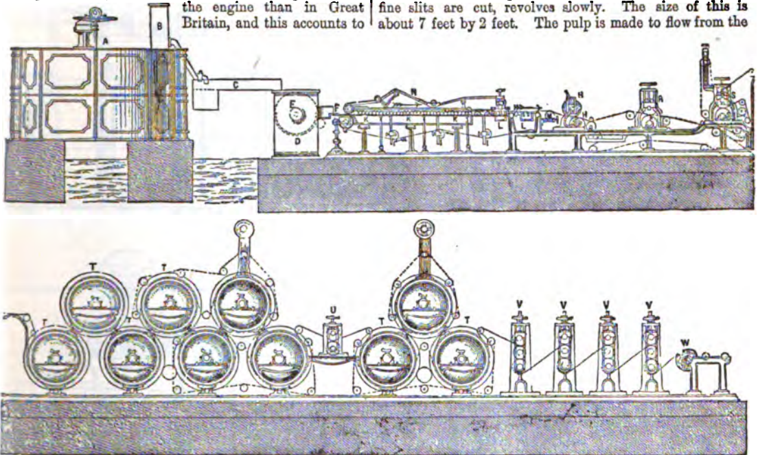
FIG. 4.—Paper Machine—Vertical Section.
