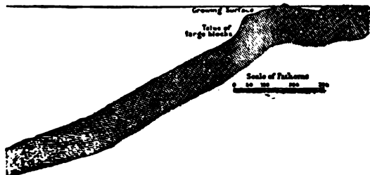
FIG. 10.—Section across the Barrier Reef, Tahiti.
