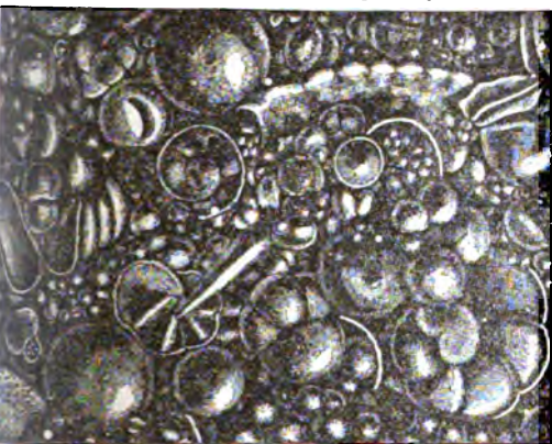
FIG. 2.— Globigerina Ooze from 1900 fathoms.
