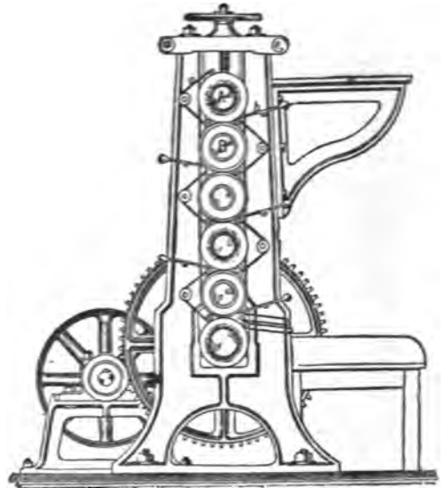
FIG. 11.—Sheet Glazing Calender.
